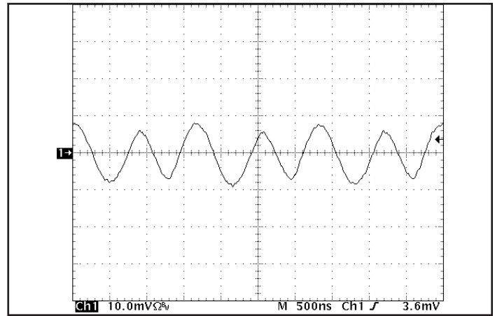
Figure 14: Input reflected ripple current, i_s , through a 10\ \mu\text{H} source inductor at nominal input voltage and rated load current ( 10\ \text{mA/div} ). See Figure 12.
